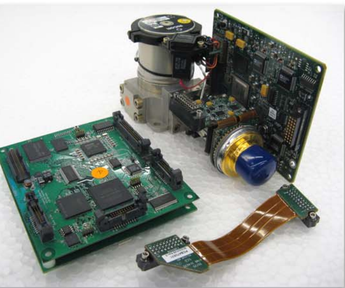
VE 1.6, detector and cooler
